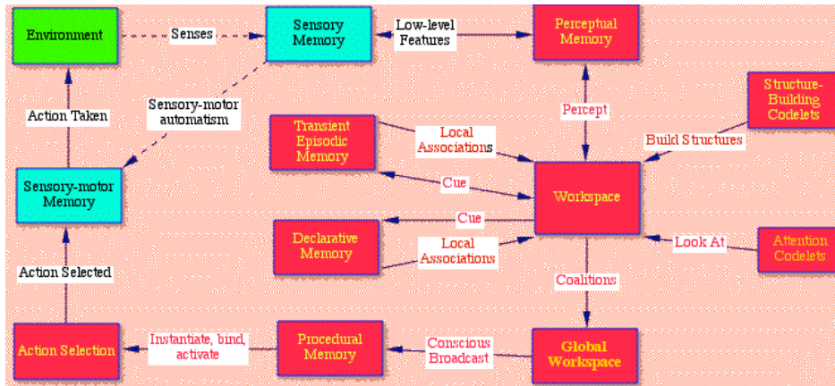
Figure 1: LIDA Cognitive Cycle Diagram
